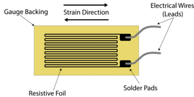
Figure 3. Construction of Strain Gauge [3]
