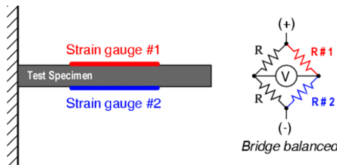
Figure 5. Half Bridge Bond Pair Strain Gauge
