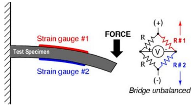
Figure 6. Downward force of on the Strain Gauge
