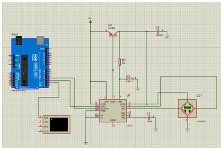
Figure 7. Connection of the Load Cell
