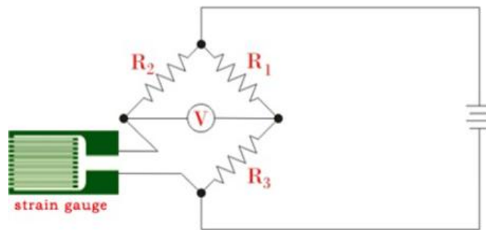
Figure 4. Wheatstone Bridge of Strain Gauge [3]
